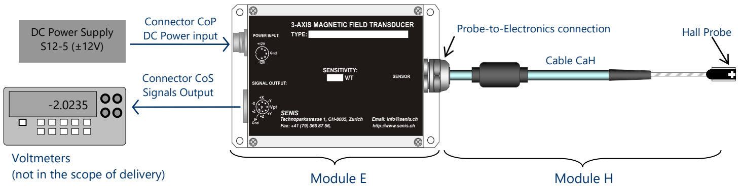
Figure 1. Typical measurement setup with a SENIS magnetic-field-to-voltage transducer with fully integrated Hall Probe (Module H) and Electronic (Module E)
