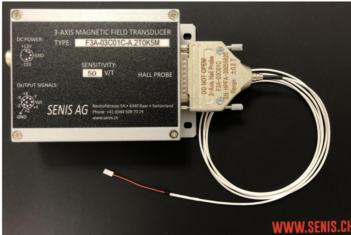
Figure 2. Photo of a 3-axis magnetic field transducer with fully integrated 3-axis Hall Probe
