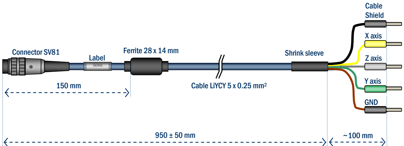
Figure 2. Dimensions and tolerances of the CO10-SE signal cable
