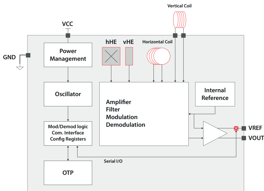
Figure 4: Block diagram of SENCS1Dx
