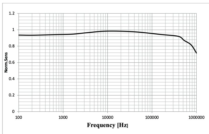
Figure 8: AC response
