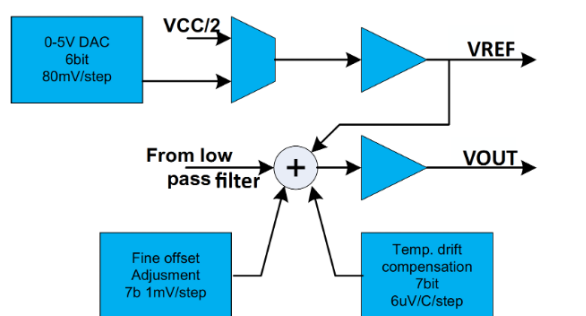
Figure 10: Signal path for VREF and VOUT
