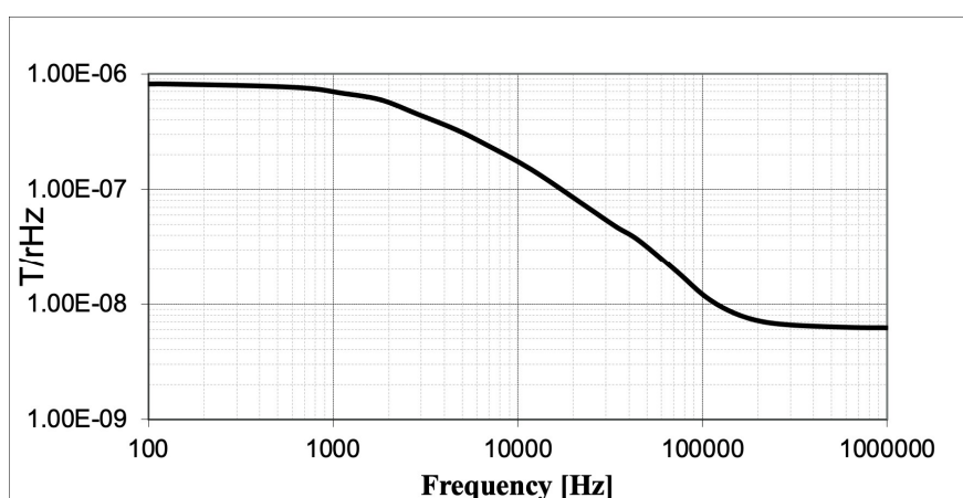
Figure 7: Equivalent magnetic field noise spectral density
