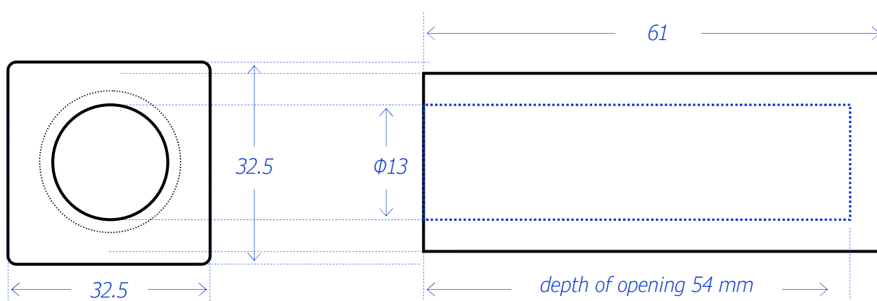
Figure 2. Dimensional drawing of the Zero Gauss chamber ZG-12-LN. All dimensions are in millimeters (mm).
