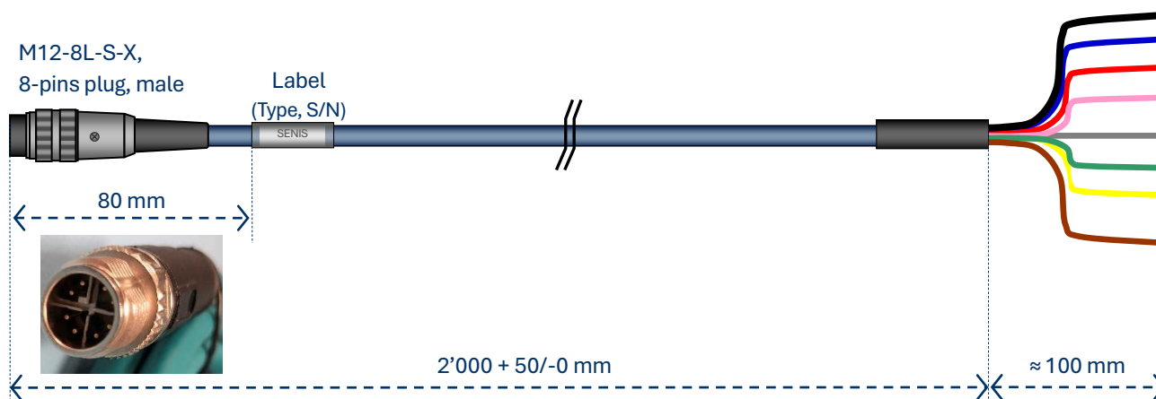
Figure 2: Dimensions and tolerances of the CO20-X signal cable
